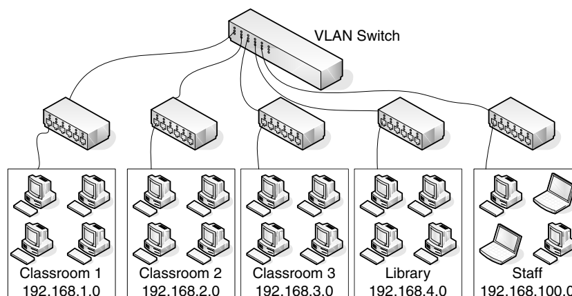
Figure 1-17 Example of a port-based VLAN
