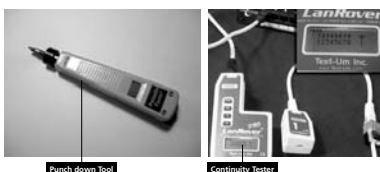
Figure 3-6 Punch down tool and continuity tester
